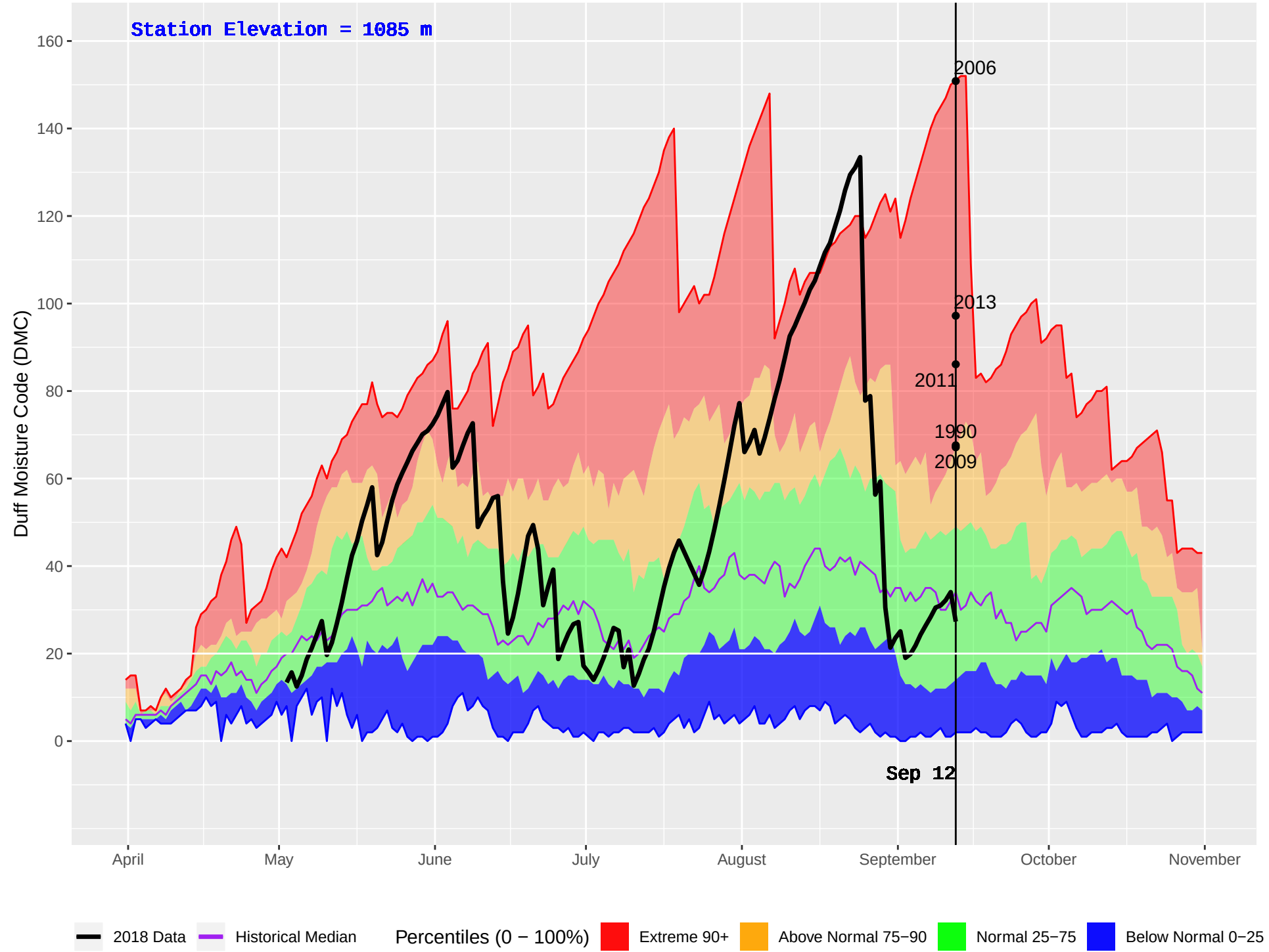
TAUTRI (206) : Historical (1970–2016) and Current (2018) Daily Duff Moisture Code (DMC)
