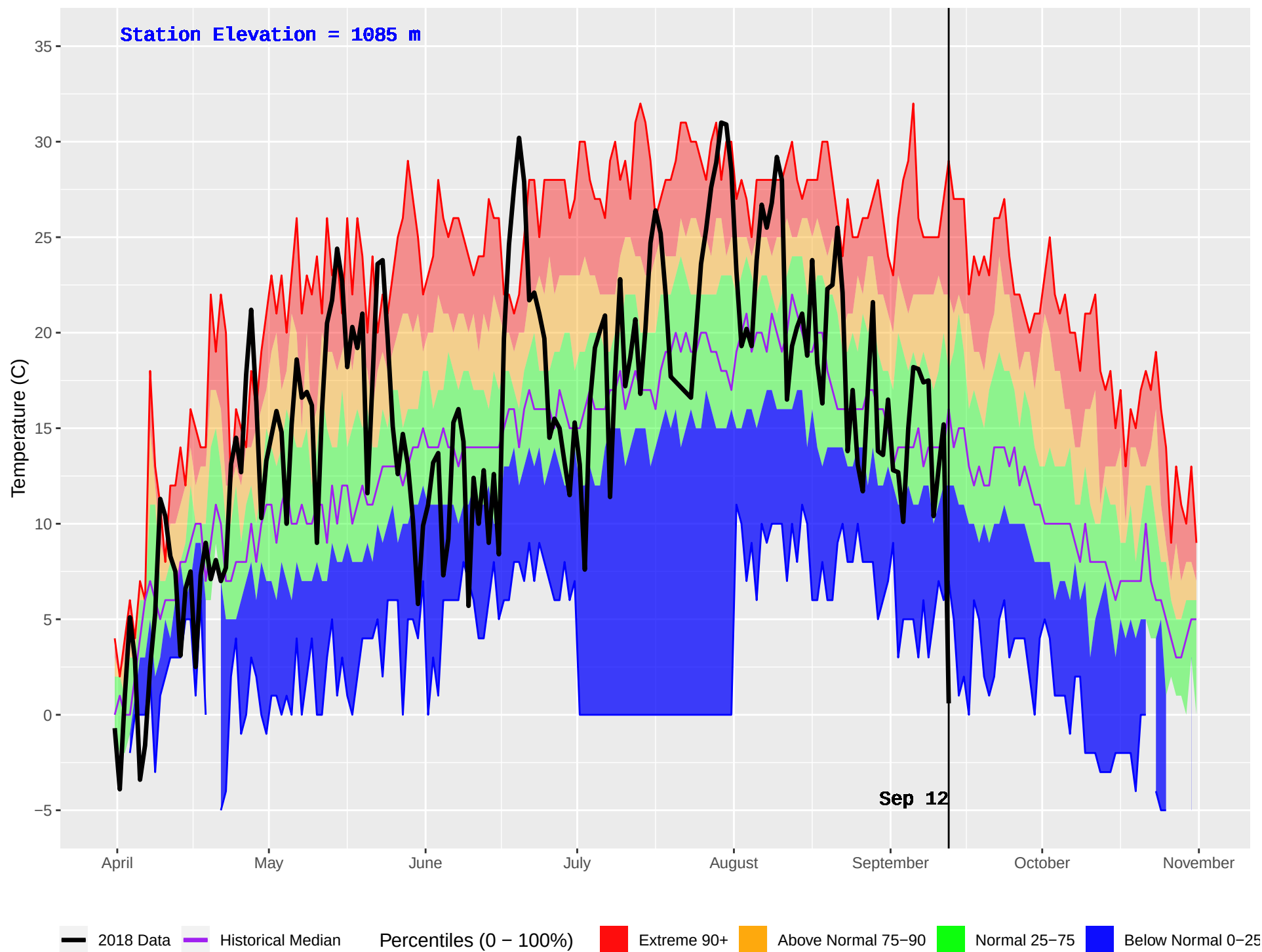
TAUTRI (206) : Historical (1970–2016) and Current (2018) Daily Temperature
