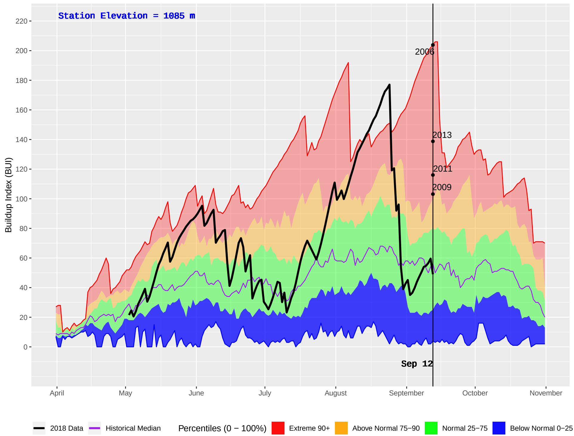
TAUTRI (206) : Historical (1970–2016) and Current (2018) Daily Buildup Index (BUI)
