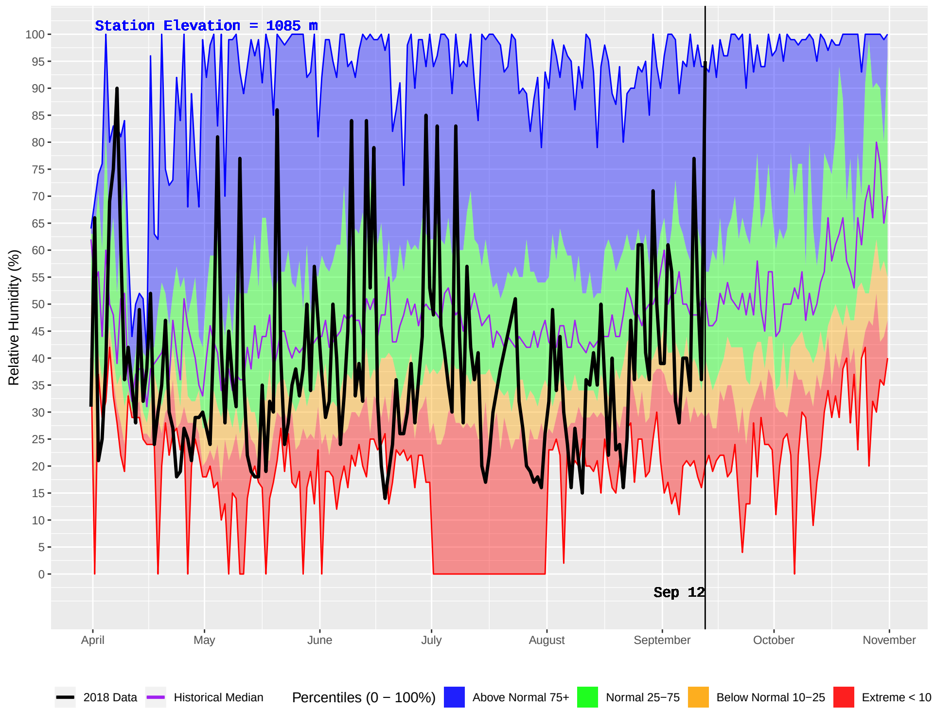
TAUTRI (206) : Historical (1970–2016) and Current (2018) Daily Relative Humidity
