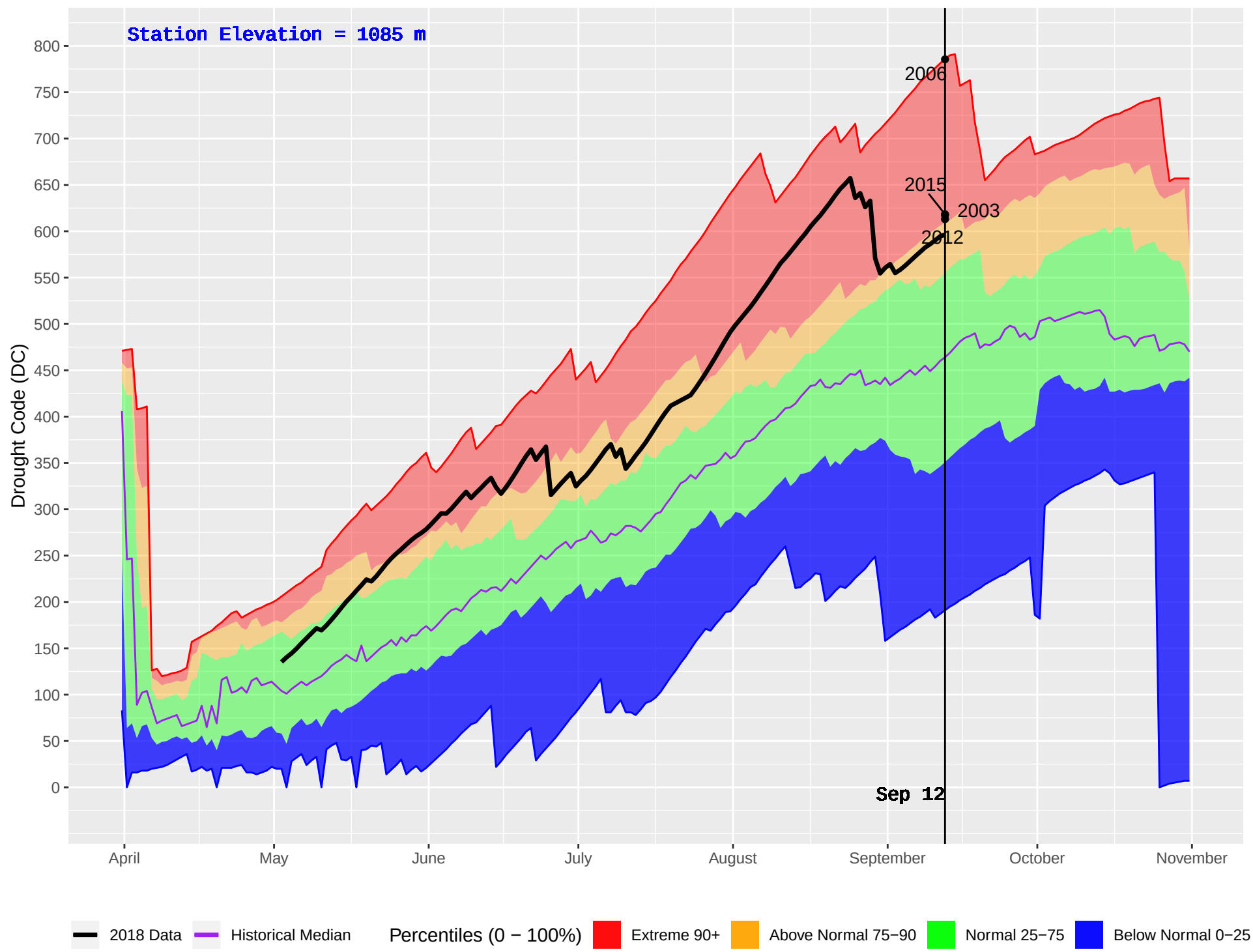
TAUTRI (206) : Historical (1970–2016) and Current (2018) Daily Drought Code (DC)
