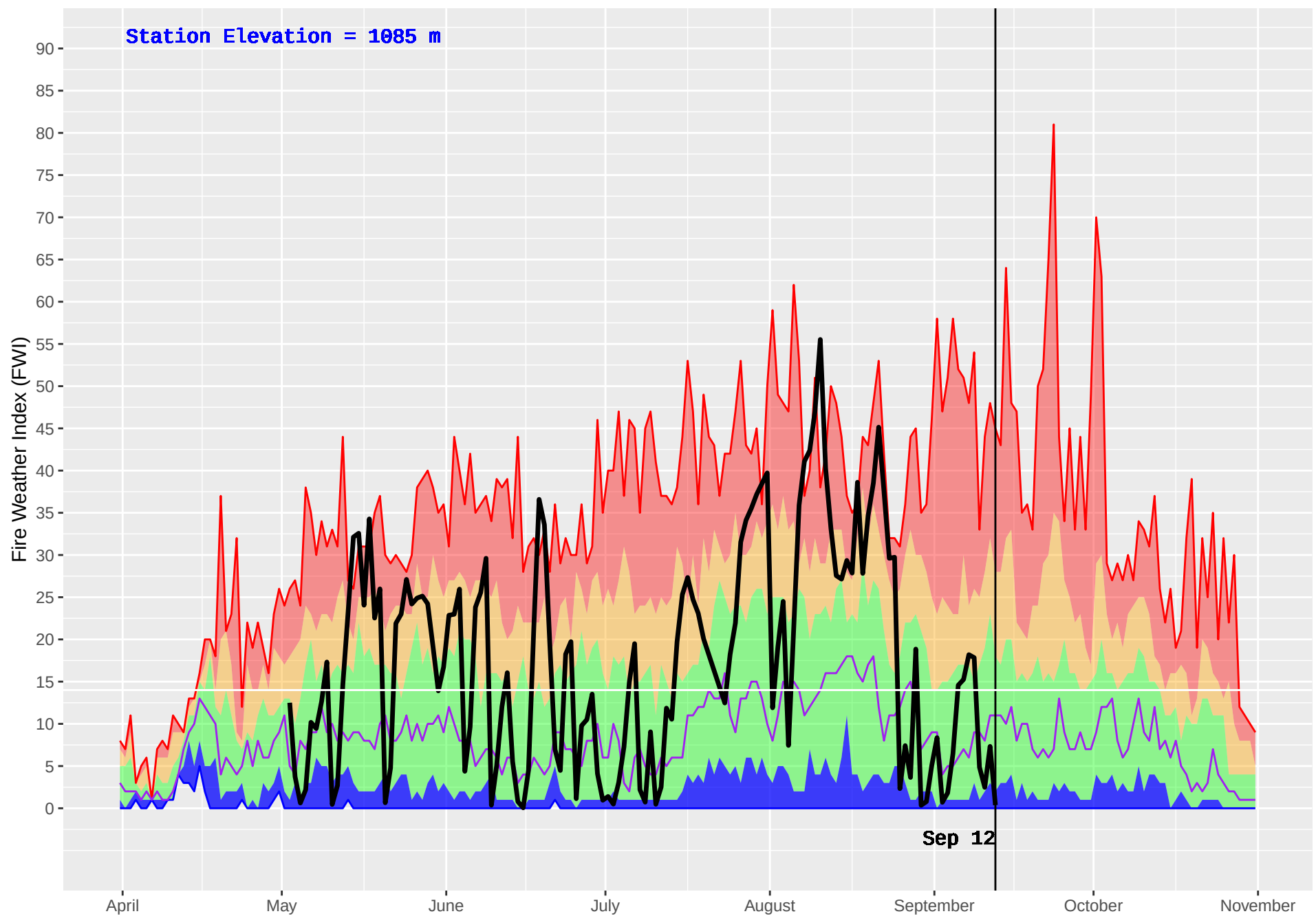
TAUTRI (206) : Historical (1970–2016) and Current (2018) Daily Fire Weather Index (FWI)
