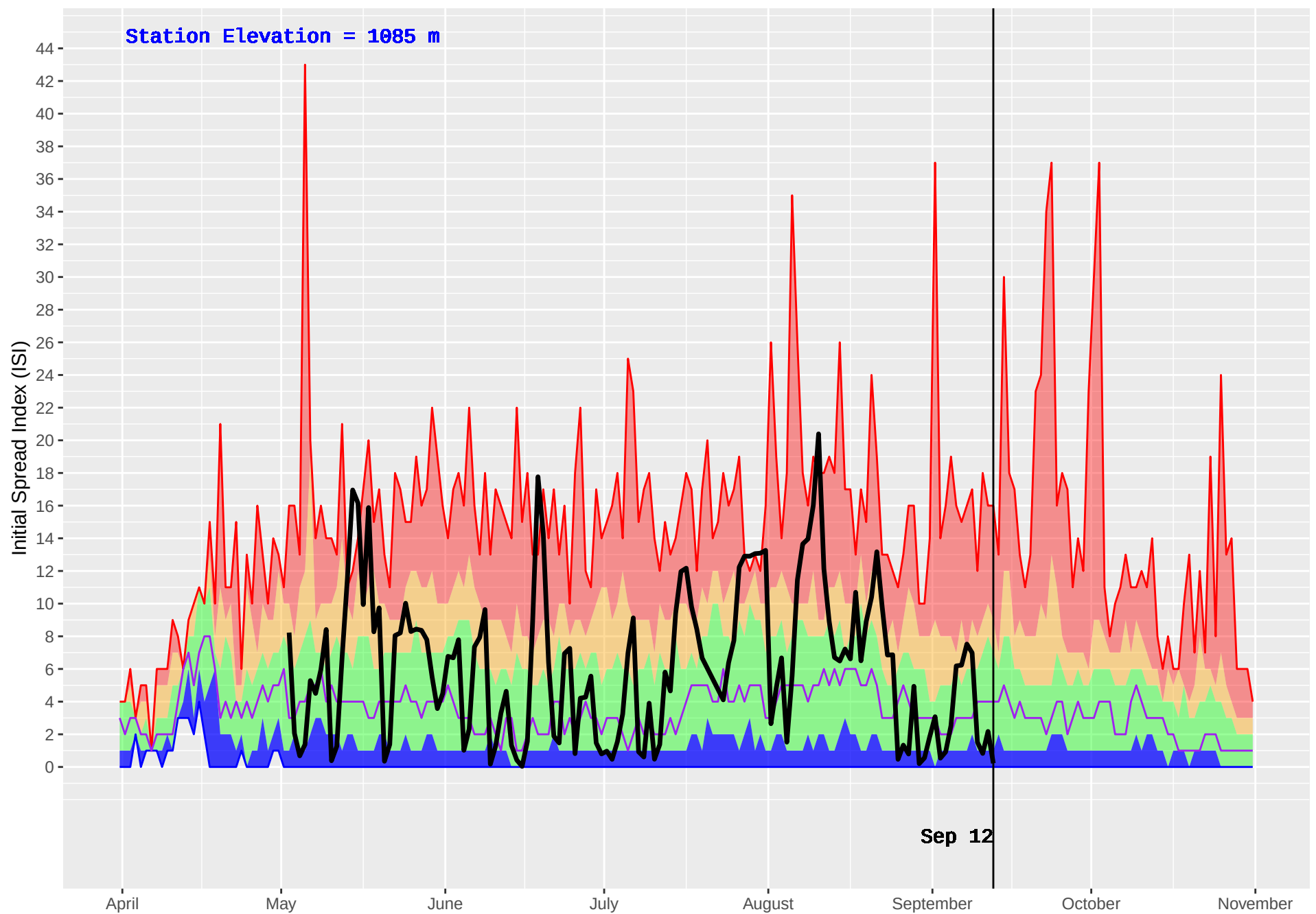
TAUTRI (206) : Historical (1970–2016) and Current (2018) Daily Initial Spread Index (ISI)
