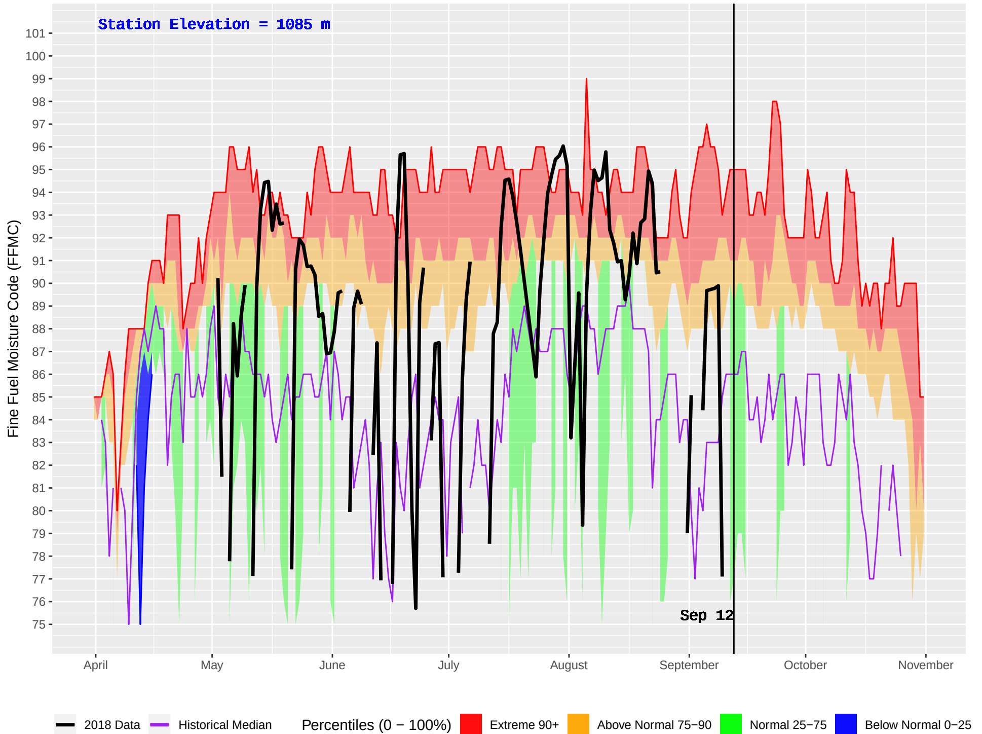
TAUTRI (206) : Historical (1970–2016) and Current (2018) Daily Fine Fuel Moisture Code (FFMC)
