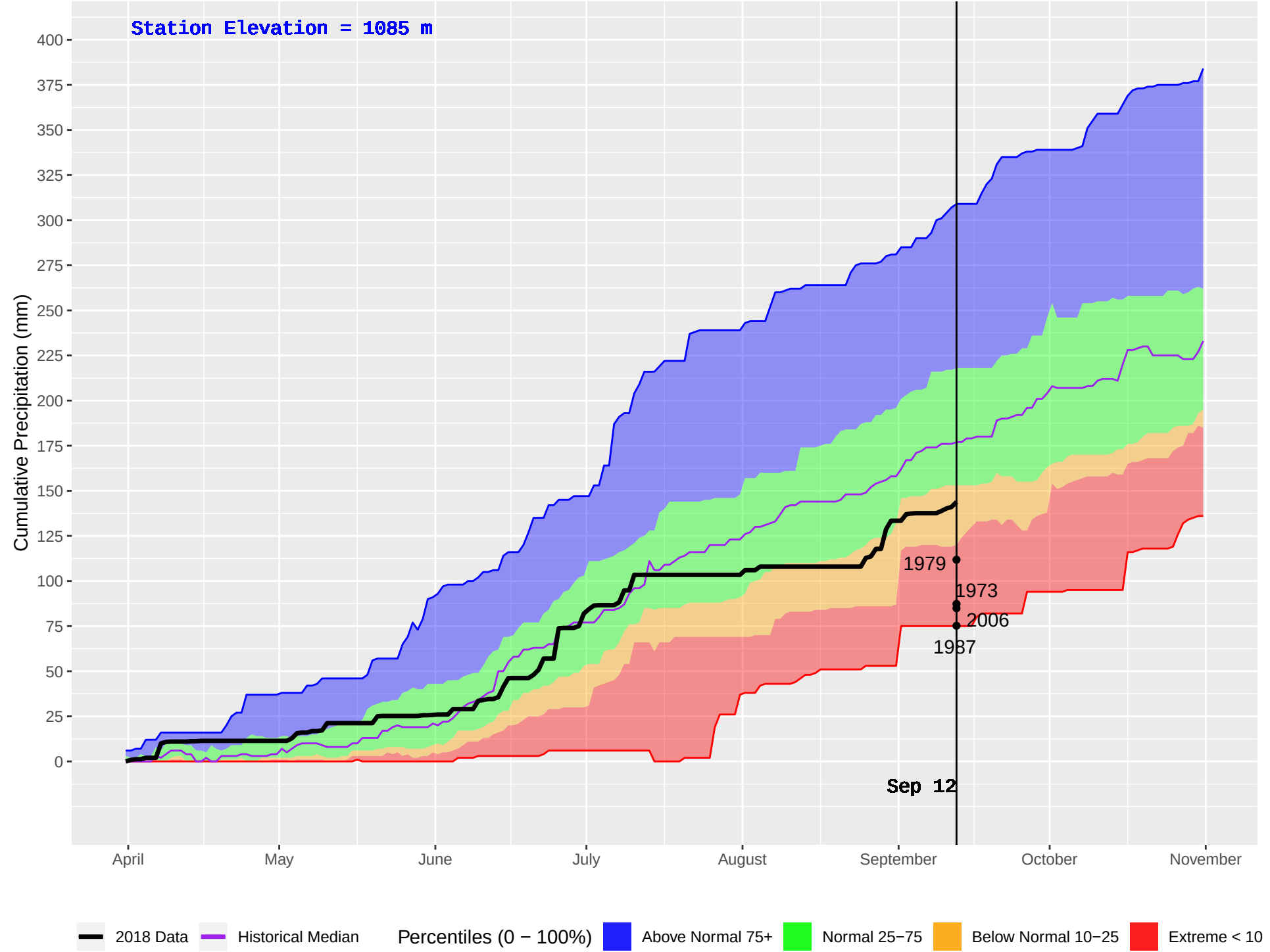
TAUTRI (206) : Historical (1970–2016) and Current (2018) Daily Cumulative Precipitation
